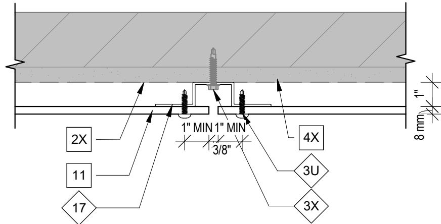
2 INOVEZE E-PLANK VERTICAL JOINT DETAIL O408 SCALE: 3" = 1'-0"
