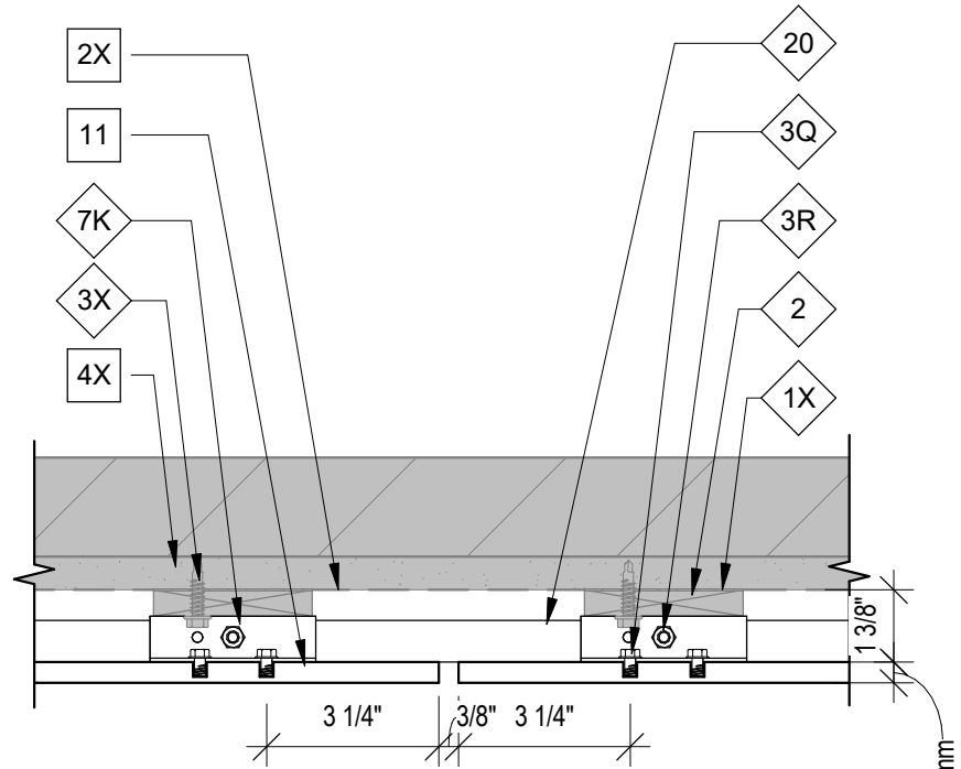
2 C2000-285 VERTICAL JOINT DETAIL O406 SCALE: 3" = 1'-0"
