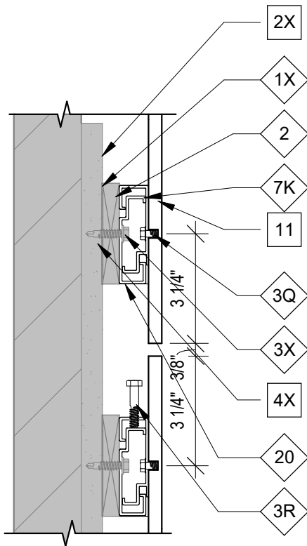
1 C2000-285 HORIZONTAL JOINT DETAIL O406 SCALE: 3" = 1'-0"
