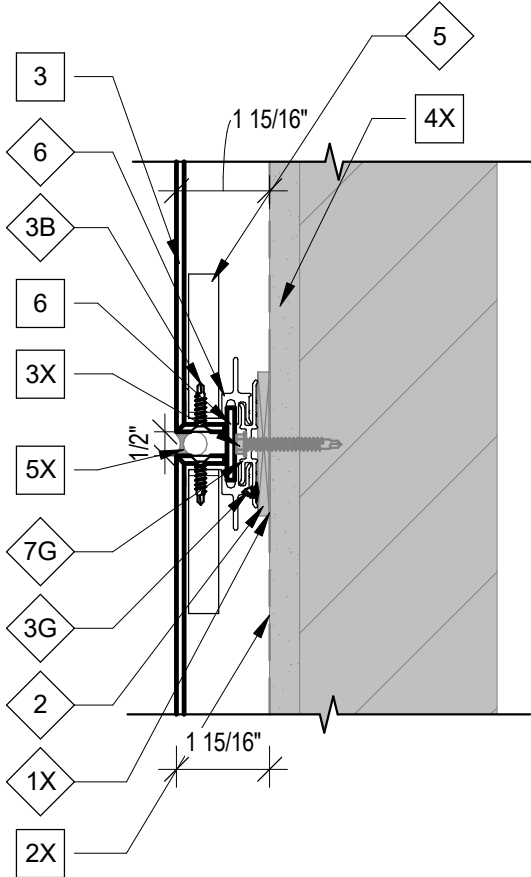
1 W5000 1/2" HORIZONTAL JOINT DETAIL O402 SCALE: 3" = 1'-0"
