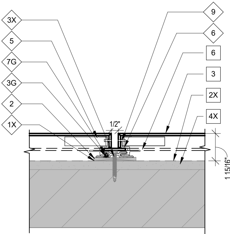
1 R4000 VERTICAL JOINT DETAIL O400 SCALE: 3" = 1'-0"
